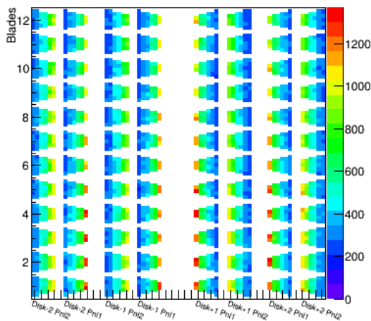
FPix Inner Shells (+x)
